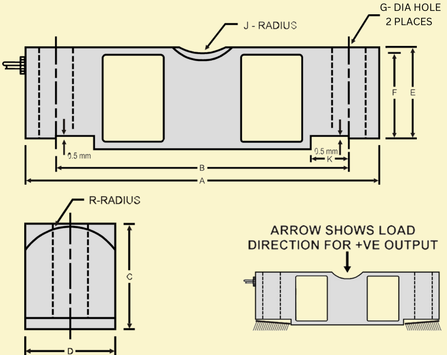
Double ended shear beam Load Cell Blueprint
