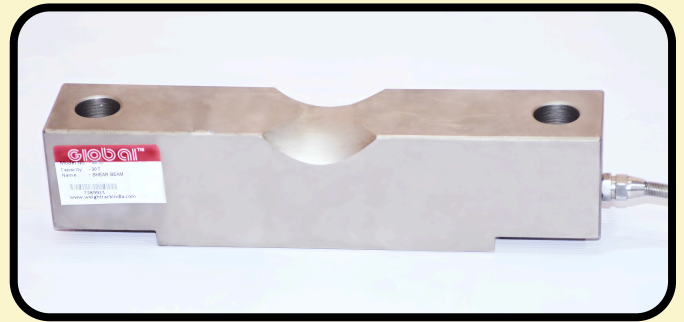
MODEL : GSB(AD) Series Double ended shear beam Load Cell
